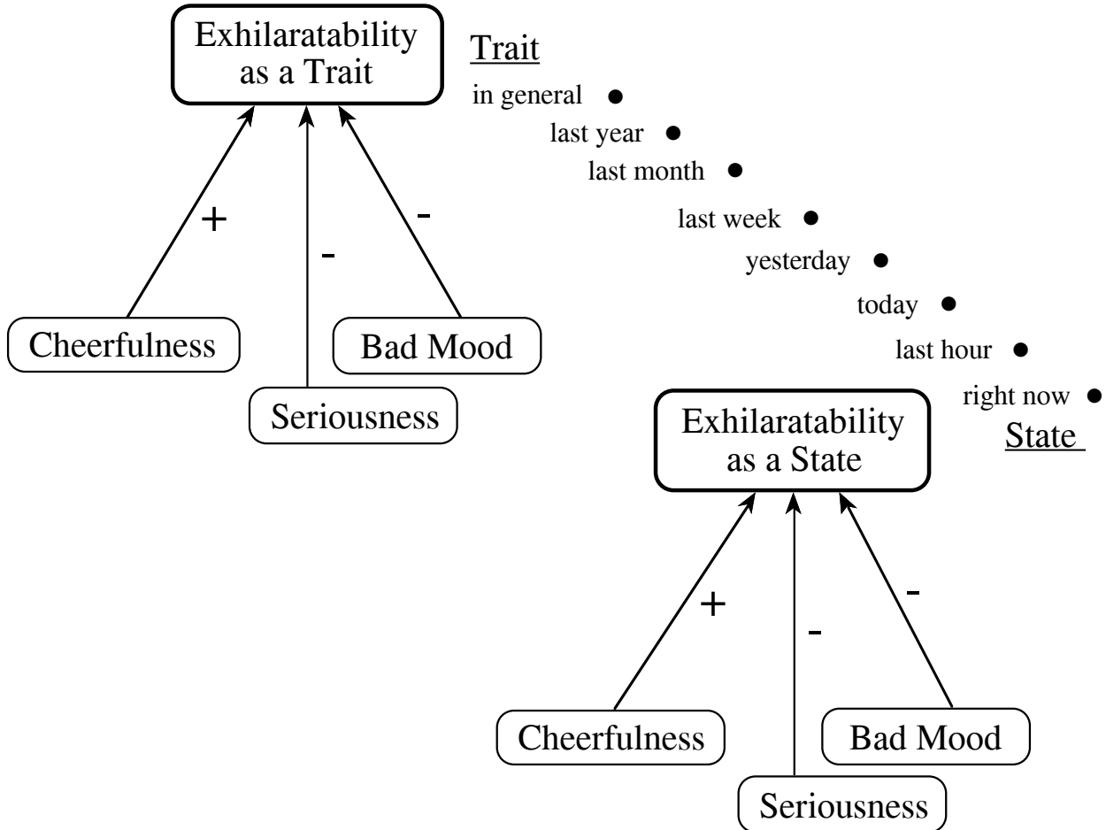
Figure 1. Hypothesized relationship between cheerfulness, seriousness, and bad mood as states and traits and exhilaratability
